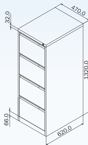
4 DRAWER V.F.C.
