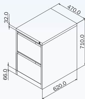
2 DRAWER V.F.C.
